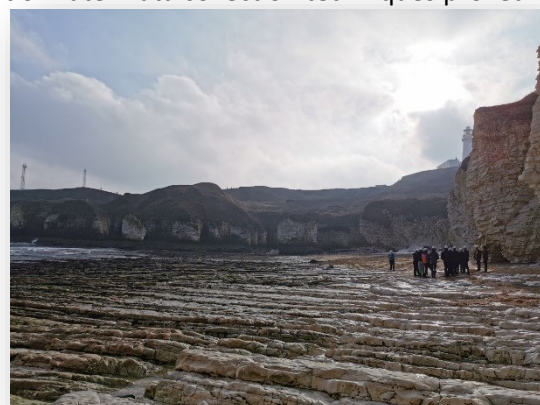
The Wave Cut Platform at Selwicks Bay
